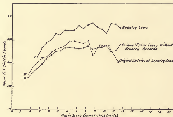
FIG. 15.—ARITHMETIC MEAN FAT YIELDS OF REGISTER-OF-MERIT JERSEY COWS (Data from Graves, U. S. D. A. Bul. No. 1352)
